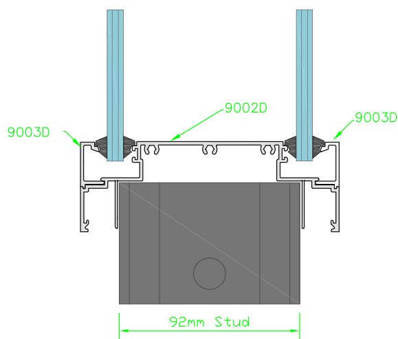
Sill to wall
