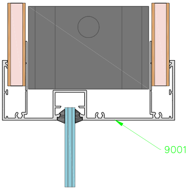
Head to wall detail
