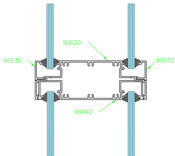
Glazed transom
