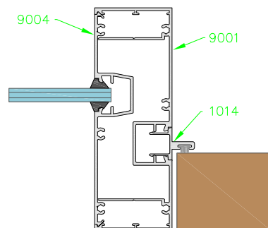
Door opening
