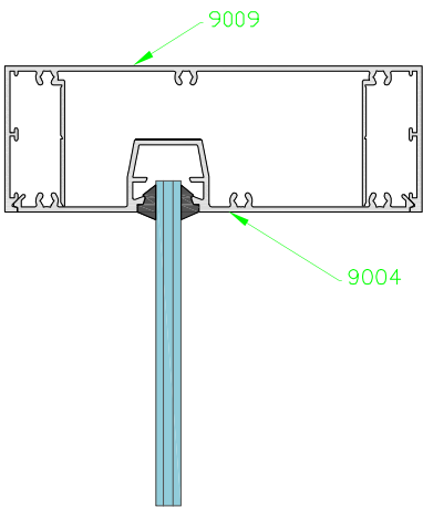
Head detail
